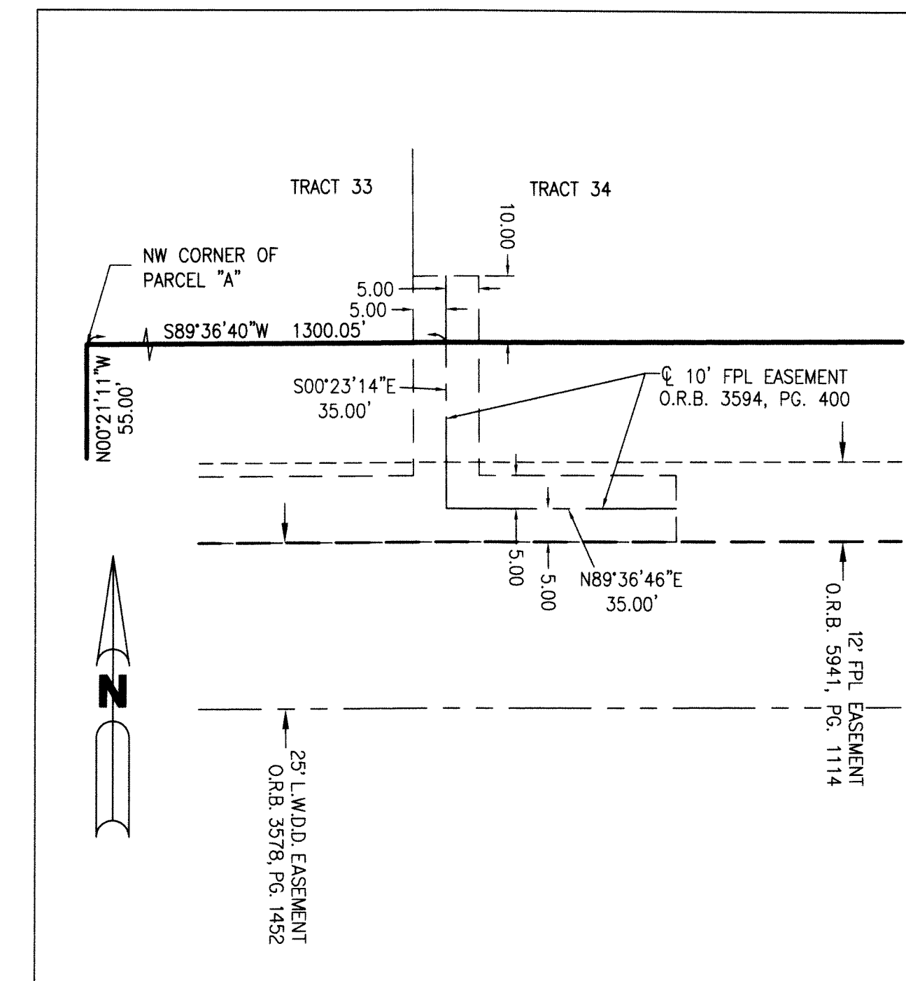
DETAIL "B" SCALE: 1"=20'
